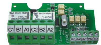
SE-EB01 I/O expansion board
