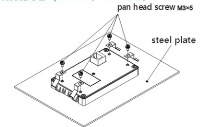
Installation package SMK301 (PU301, PU301C)
