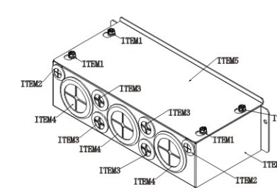
Frame E/F E:WBK302 F:WBK303
