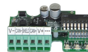
SE2-DN01 Device-Net communication expansion board
